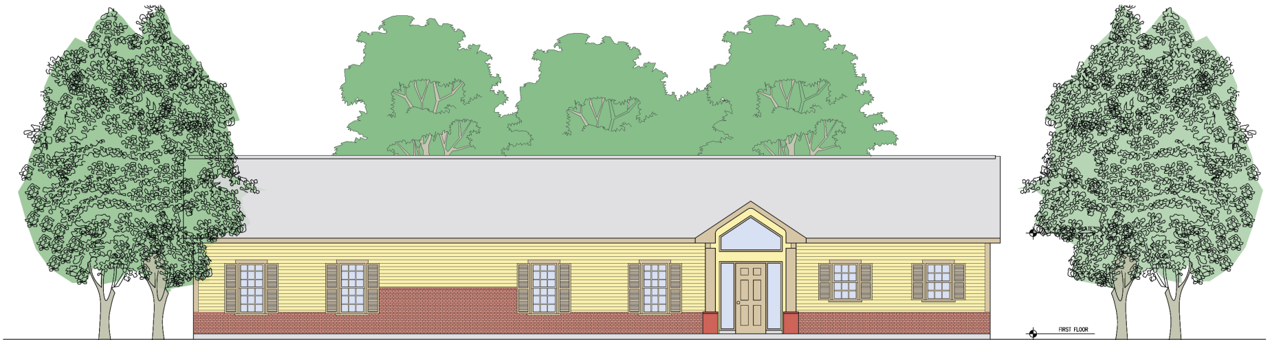
1 FRONT ELEVATION 1/4" = 1'-0"
